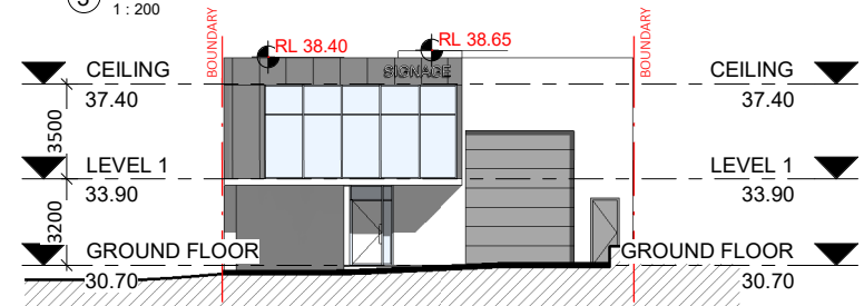
4 NP - SOUTH EAST ELEVATION 1 : 200
