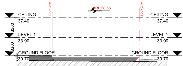
3 NP - NORTH WEST ELEVATION 1 : 200
